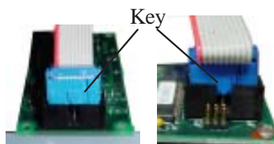
Expansion Port for Temperature Display: Uses I 2 C Communication
