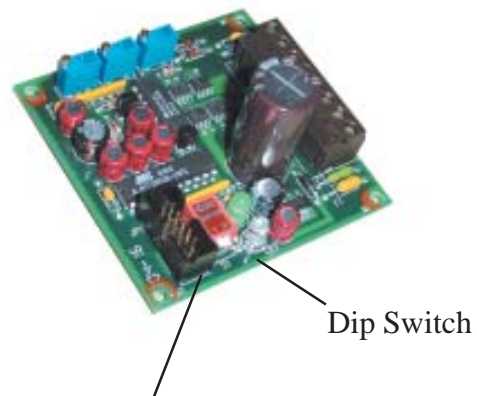
Expansion Port for Temperature Display: Uses I 2 C Communication
